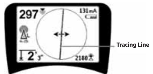
Figure 19: Tracing Line Showing Low Distortion
